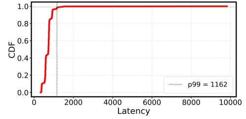
Figure 3: CDF of PCIe write latency between the compute node and the FPGA controller, with 99 th percentile latency of 1162 ns and average latency of 694 ns.
