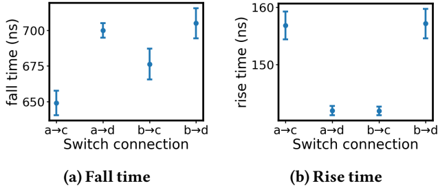
Figure 6: Electrical-to-Optical rise/fall time for different switch configurations: a \rightarrow c & b \rightarrow d represent bar connection and a \rightarrow d & b \rightarrow c represent the cross connection.
