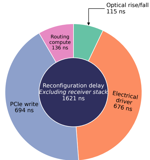
Figure 1: Reconfiguration delay breakdown excluding receiver locking, with optical rise/fall time contributing only 7%.
