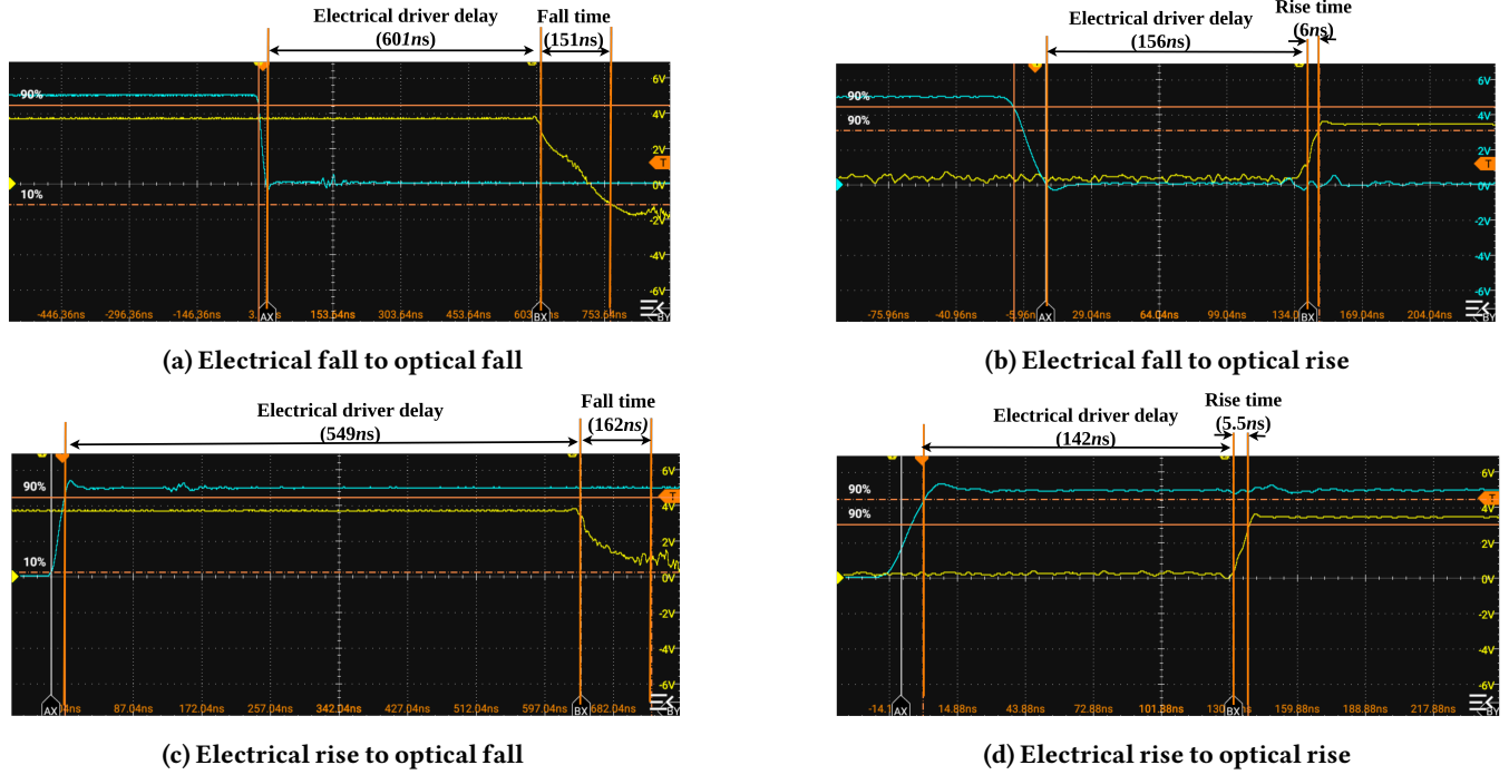
Figure 7: Measured transition delays for a 2 \times 2 optical switching element: While the intrinsic optical switching latency is approximately 150 ns, the electrical-to-optical response time reaches up to 600 ns, making the driver and actuation path a non-negligible contributor to the overall reconfiguration delay.
