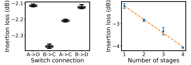
(a) Insertion loss of a switch (b) Insertion loss with Scaling
