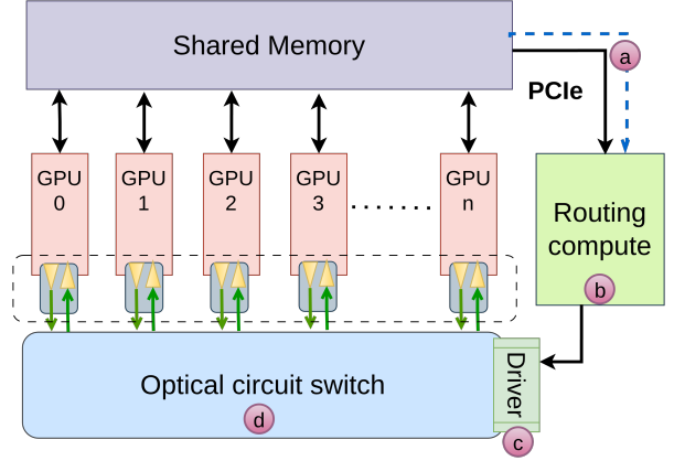
Figure 2: Hardware prototype
